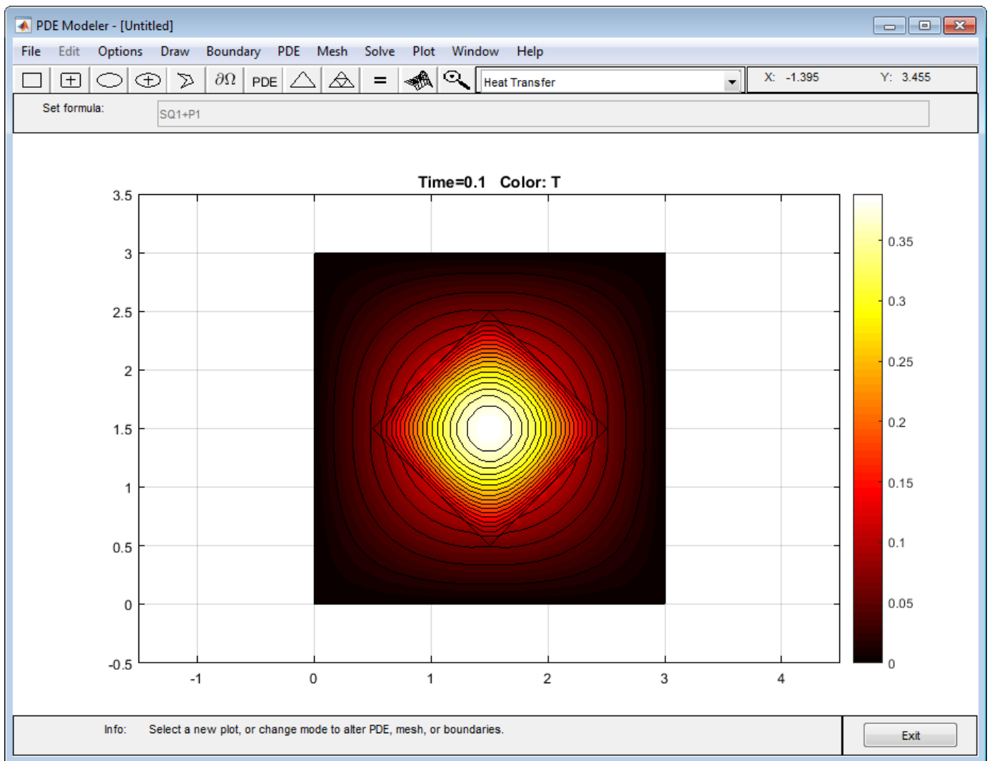
Isothermal Lines
