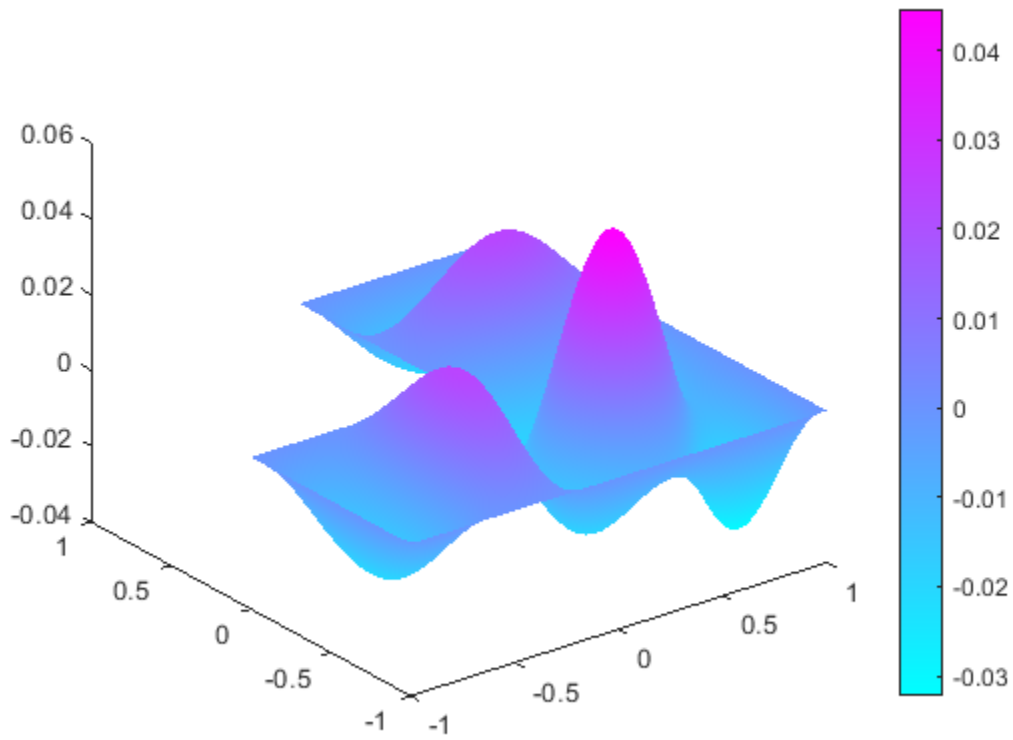
figure membrane(12,20,9,9)
