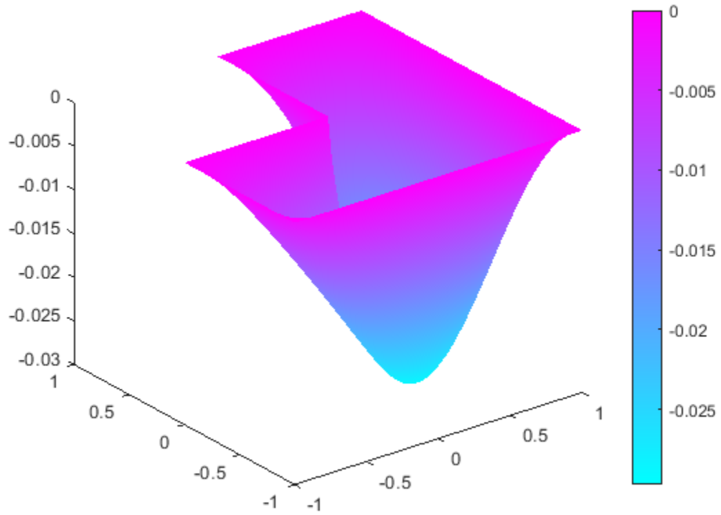
figure membrane(1,20,9,9)
